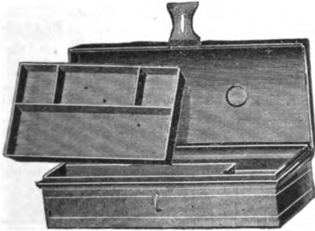
No. 20. Tin, Dark Japan Finish, size 10\frac{1}{2} \times 4\frac{1}{2} \times 3 in.; has one tray and space for tackle.....$1.00 each.
